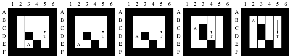
Figure 2: Moving-Target Search
