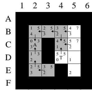
Figure 7: A*
