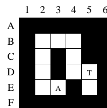
Figure 1: Gridworld
