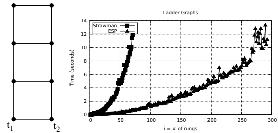
Figure 2: Runtime on ladder graphs
