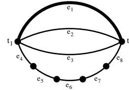
Figure 1: Series-parallel graph
