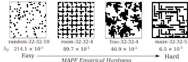
Figure 1: Example maps and their \lambda_2
