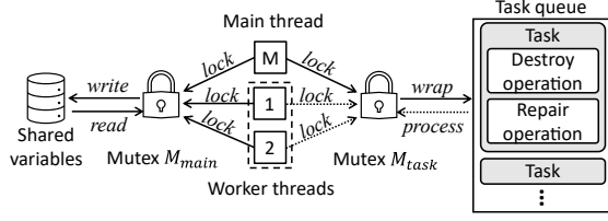
Fig. 2. Illustrative example of the DROP-LNS framework with a main thread “M” and two worker threads “1” and “2”. Arrows are the actions from each thread.
